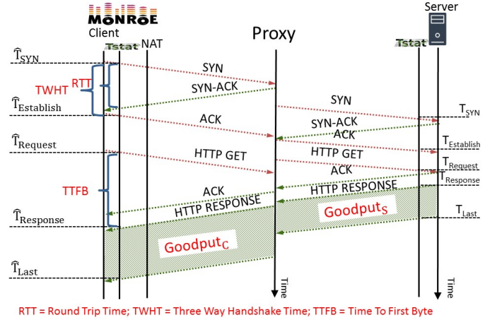
Fig. 3: Packet timeline in case of PEP in the path
