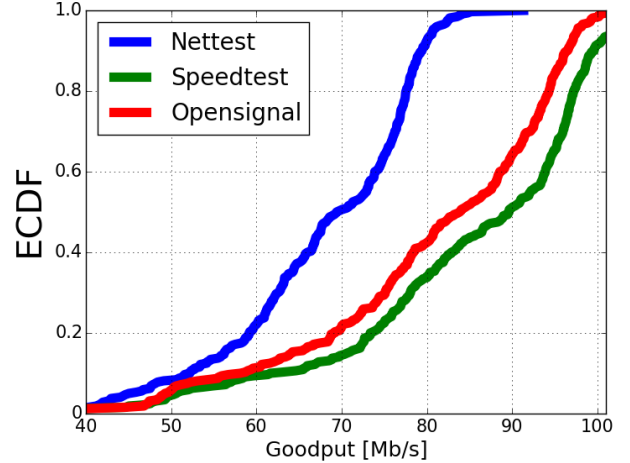
Fig. 1: ECDF of reported download rate for different tools in 4G
