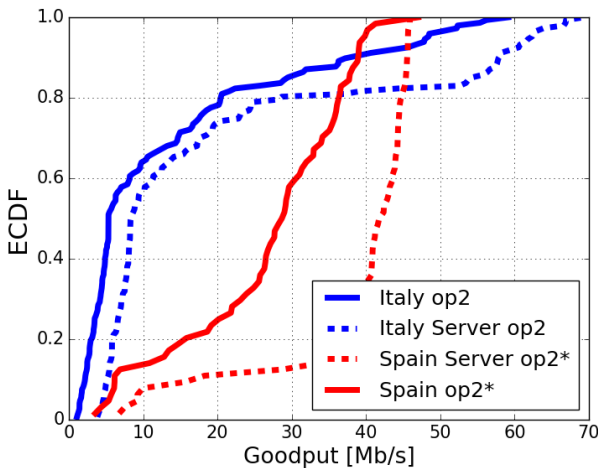
Fig. 11: Goodput experienced from client and server sides for the same operator SIM in Italy and Spain
