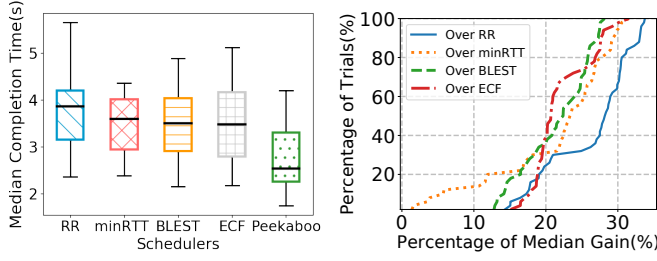
Figure 7. File download performance of Peekaboo and other schedulers.
