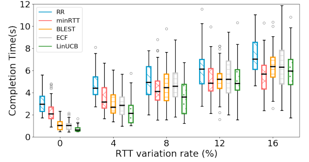
(b) Performance under different RTT variations
