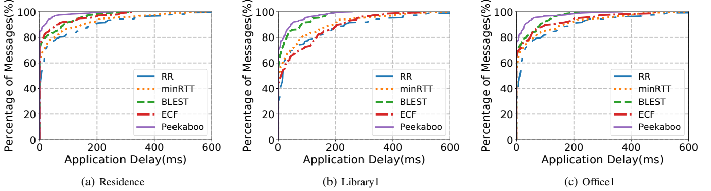
Figure 12. Real-time streaming at 2 Mbps at different scenarios.
